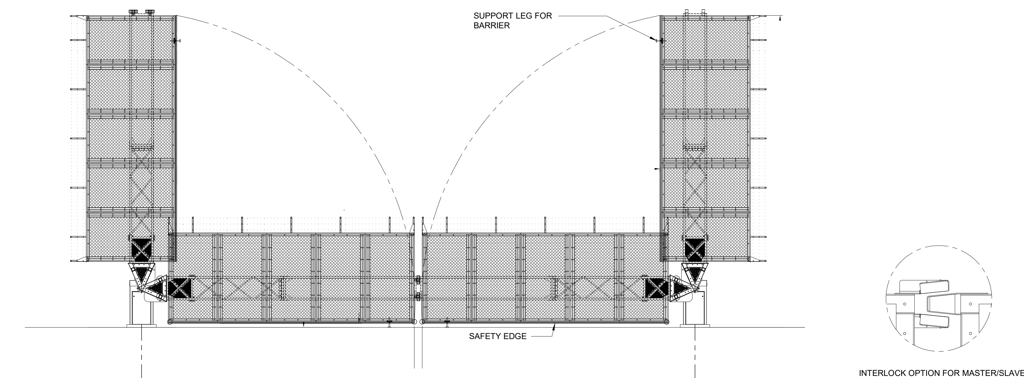
3 VEHICLE DOUBLE GATE DETAILS TY703 1:2
