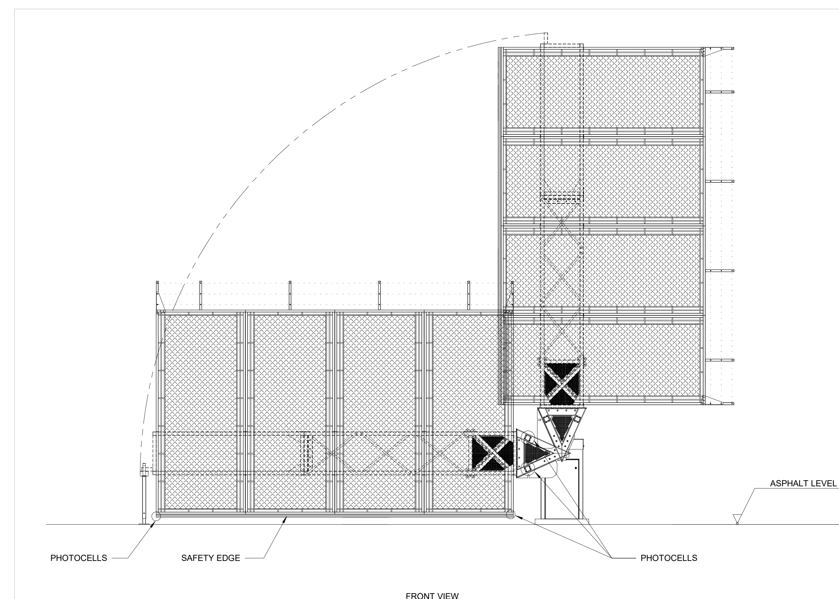
4 VEHICLE GATE DETAILS TY703 NTS
