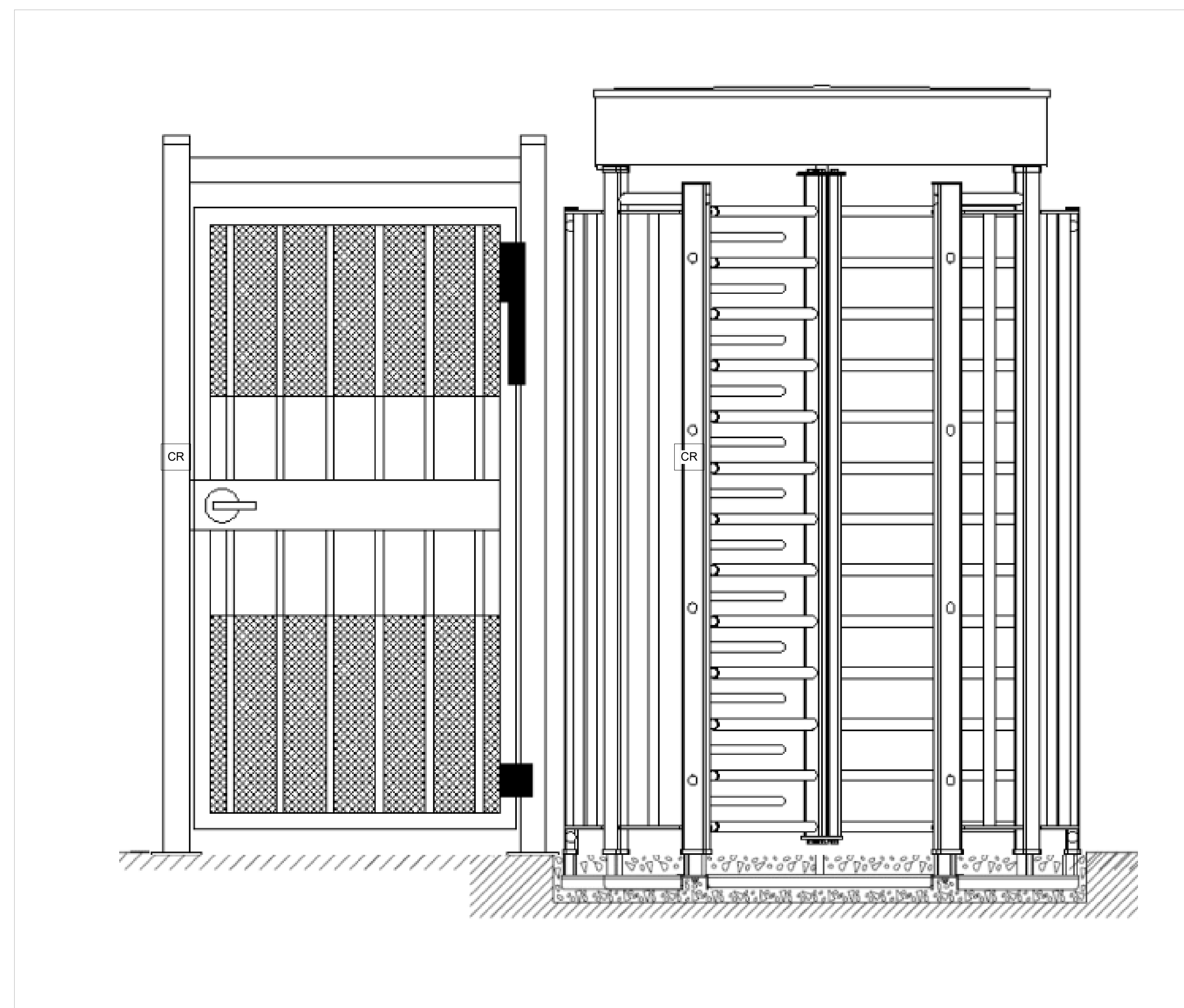
2 TYPICAL AMERICANS WITH DISABILITIES ACT (ADA) GATE DETAILS TY703 NTS
