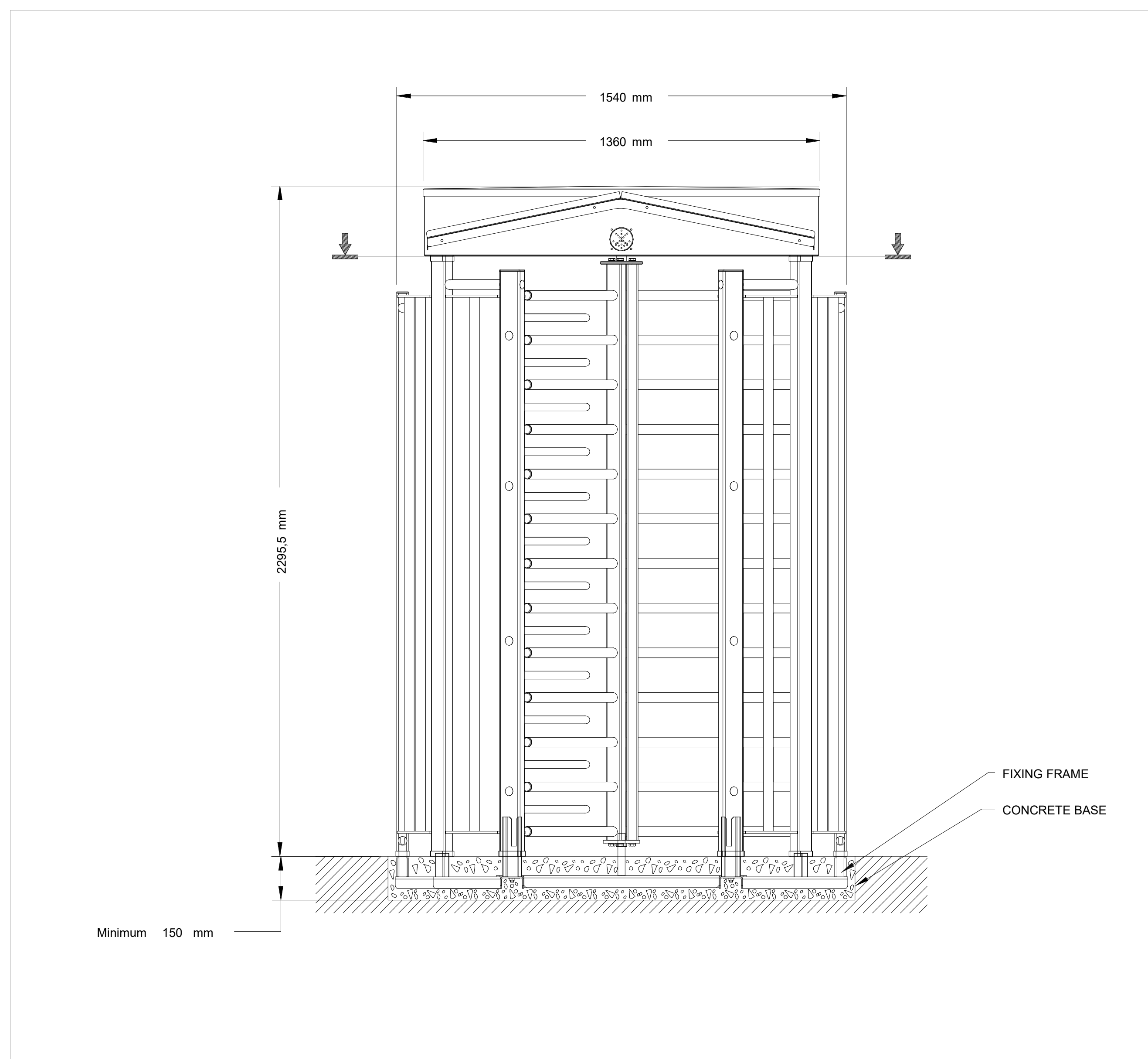
1 TYPICAL TURNSTILE GATE DETAILS TY703 NTS
